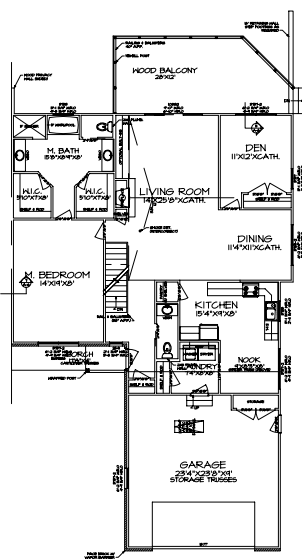
FIRST FLOOR PLAN (UNIT A) SCALE: 1/4"=1'-0"
