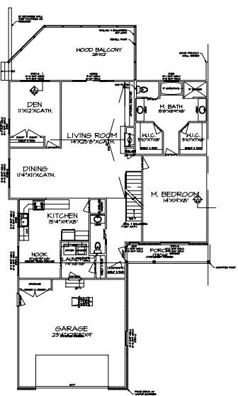
FIRST FLOOR PLAN (UNIT B) SCALE: 1/4"=1'-0"
