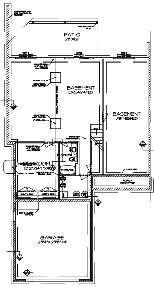
FOUNDATION PLAN (UNIT B) SCALE: 1/4"=1'-0"
