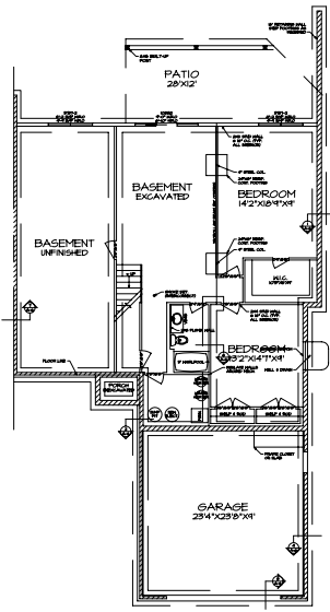
FOUNDATION PLAN (UNIT A) SCALE: 1/4"=1'-0"
